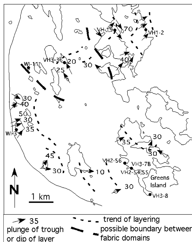
Fig. 3 Geologic map of the western half of the Vinalhaven granite, showing the occurrence of planar and trough schlieren and locations for all illustrated schlieren
