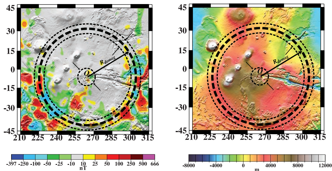
Figure 1. Maps showing (left) radial magnetic field anomalies B_r , after Langlais et al. [2004] and (right) topography from Mars Orbiting Laser Altimetry (MOLA) data for the Tharsis region. Whereas strong magnetic fields occur below 6–7 km in the southern half of the approximately axisymmetric bulge, virtually no magnetic fields are observed at higher elevations. Thick lines indicate the radius of the demagnetized region as defined from the center of the topographic bulge O (small dashed circle). Thin lines indicate the uncertainties on the center of the bulge and on the radius of the demagnetized region. The absence of magnetized crust north of the dichotomy boundary is discussed in the text.
