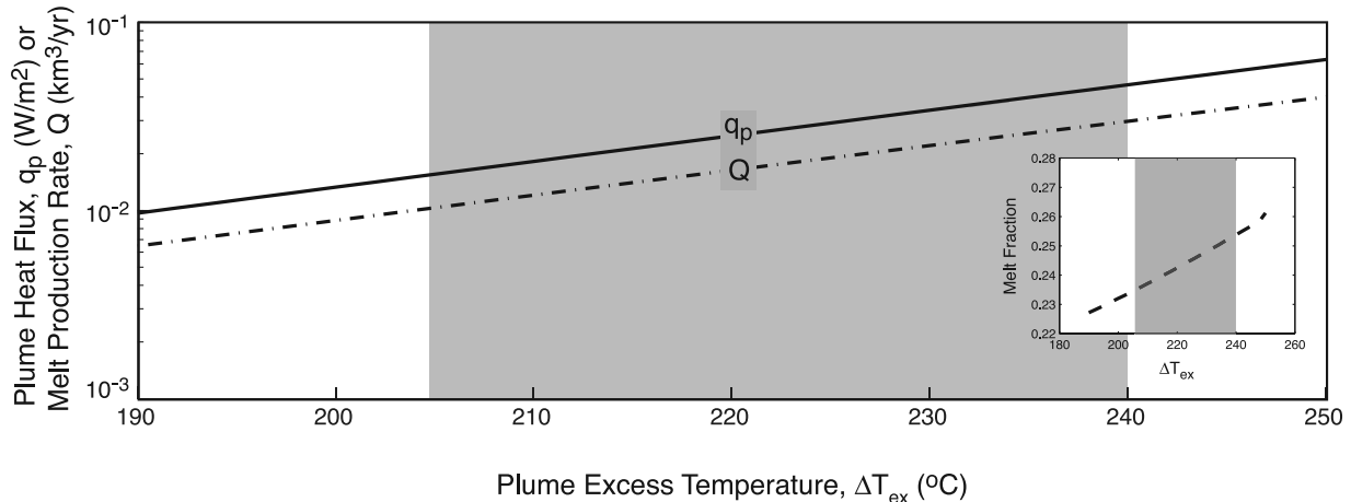
Figure 6. Plot showing the plume heat flux q (solid line), melt production rate Q (dash-dotted line), and mantle melt fraction (inset) as a function of maximum plume excess temperature \Delta T_{max} .
