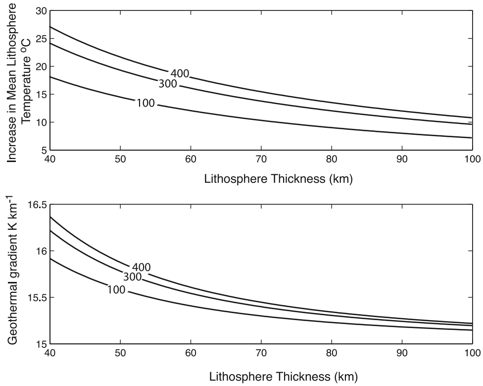
Figure 3. Plots showing (top) the increase in the mean temperature and (bottom) geothermal gradient in the lithosphere as a function of initial plume excess temperature. Calculations assume thermal conduction to the lithosphere over the time for a plume head to spread to one half its initial height (see text for discussion).
