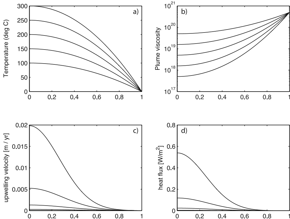
Figure 4. Plots indicating the (a) temperature, (b) viscosity, (c) upwelling velocity, and (d) heat flux as a function of radial position in the active part of the model plume conduit.
