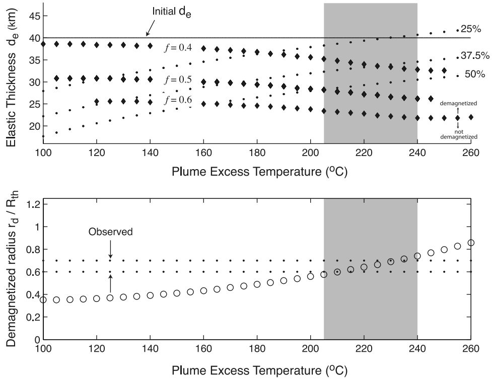
Figure 5. (top) The predicted elastic thickness d_e as a function of maximum plume excess temperature \Delta T_{ex} for a range of f - h_t conditions, assuming that d_m = d_e = 0.4d_L . Dots indicate elastic thicknesses determined from considerations of the flexural response of the lithosphere to an underlying mantle plume conduit. Solid diamonds indicate the minimum value for d_e at which the crust will appear demagnetized to an orbiting MGS satellite. (bottom) The normalized radius of the demagnetized region as a function of plume excess temperature. Open circles are values predicted on the basis of the analysis of the spreading of a mantle starting plume head beneath a rigid lithosphere in section 2.2.1. Dots are observations determined from Figure 1. The region shaded in grey indicates the range in excess temperatures for which the expected demagnetized radius is consistent with observations. See text for discussion.
