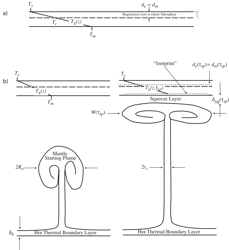
Figure 2. Definition sketches for each component of our model. (a) The initial (pre-Tharsis) thermal and magnetic state of the lithosphere. The dashed line indicates the depth of the magnetized crust, which is taken to be approximately equal to the elastic thickness. (b) The rise and time-dependent spread of a mantle starting plume beneath the Martian lithosphere. The topographic “footprint” is an expected result of thermomechanical erosion of the lithosphere on spreading of the plume head over the time to thin to about one half its initial diameter. The dotted line indicates a corresponding shallowing of the Curie isotherm in response to the transient conduction of heat from the plume head to and across the lithosphere. (c) A steady state thermal model of a Martian mantle plume conduit under steady state conditions. (d) A model for the flexural response of the lithosphere to the buoyancy force imparted by an underlying plume conduit. See text for discussion and Table 1 for notation.
