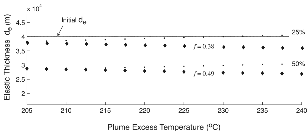
Figure 7. Plot showing the expected elastic thicknesses over a range of f - h_t conditions for 205 \leq \Delta T_{ex} \leq 240^\circ\text{C} , the preferred excess temperatures identified in Figure 5 (bottom). Dots indicate elastic thicknesses determined from considerations of the flexural response of the lithosphere to an underlying mantle plume conduit. Solid diamonds indicate the minimum value for d_e at which the crust will appear demagnetized to an orbiting MGS satellite.
