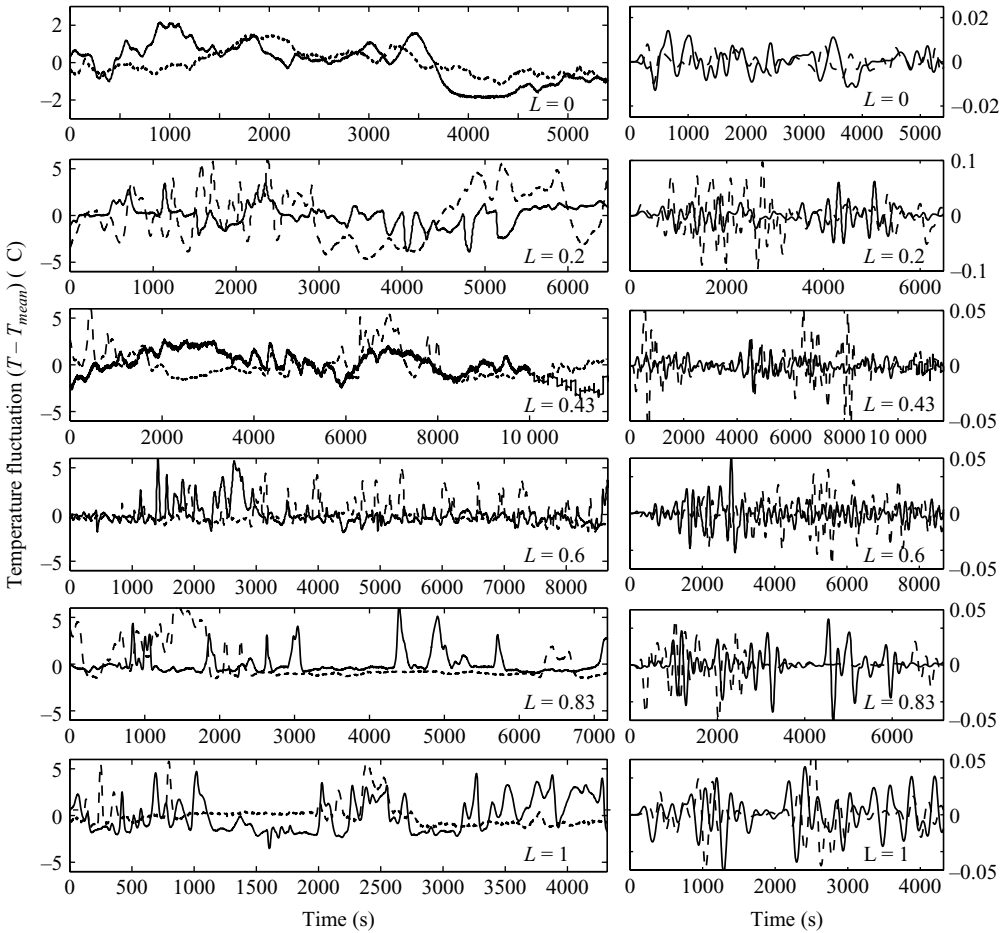
FIGURE 4. Plots showing time series of temperature variations about the mean temperature of the hot thermal boundary layer recorded by thermocouples ‘TC1’ (solid line) and ‘TC2’ (dashed line) (left panel). Also shown are the same data after it has been low pass filtered and differenced such that the contributions of thermals to the signal in each regime emerges more clearly (right panel).
