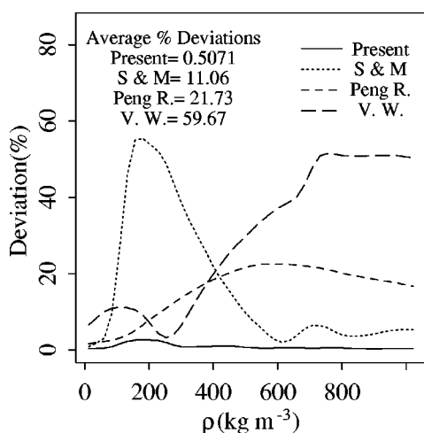
FIG. 3. Comparison of the predictive accuracy of four equations of state. The 1486 p - V - T values are from Haar et al. (Ref. 42) in the range 0 < T < 1200 \text{ }^\circ\text{C} , 0.1 < p < 3000 \text{ bar} , 0.16 < \rho < 1025 \text{ kg m}^{-3} . Data was binned (bin width = 24 \text{ kg m}^{-3} ), and rms percentage deviations of the predicted density calculated and smoothed.
