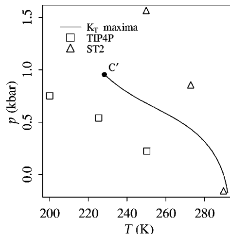
FIG. 11. Comparison of isothermal compressibility ( K_T ) maxima between the new equation of state of water, and the ST2 and TIP4P potentials (Ref. 35). The line of K_T maxima exhibits a smooth transition from ST2 like behavior near p = 0 \text{ kbar} to TIP4P behavior at higher pressures, ending in a second critical point (C').
