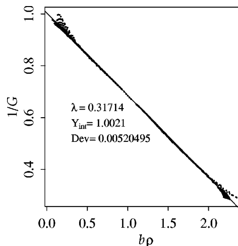
FIG. 4. 1/G vs b\rho as in Fig. 2. 1256 p - V - T values are from Haar et al. (Ref. 42) in the range 0 < T < 1200 \text{ }^\circ\text{C} , 0.1 < p < 3000 \text{ bar} , 100 < \rho < 1109 \text{ kg m}^{-3} . Supercooled data (245 points) is from Hare and Sorensen (Ref. 14) and Petit et al. (Ref. 15) in the range -34 < T < 0 \text{ }^\circ\text{C} , 1 < p < 500 \text{ bar} . The split in the data in the bottom-right corner of the figure is the result of water's density anomaly.
