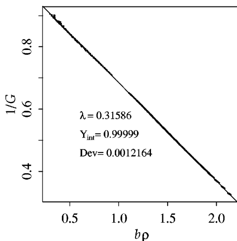
FIG. 2. 1/G vs b\rho using Eqs. (18), (19), and the p - V - T data of Fig. 1. Also shown is a best fit straight line with slope \lambda , y -intercept Y_{\text{int}} and rms deviation, Dev.
